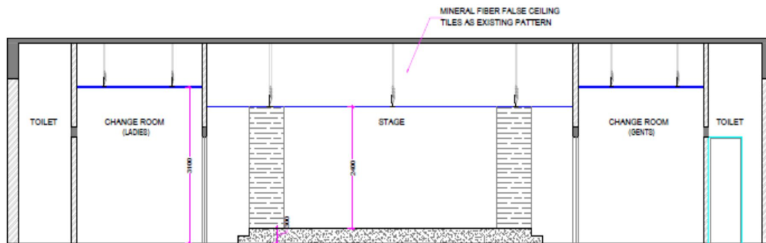
SECTION AT (X-X)
