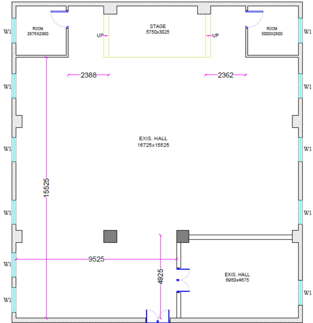
EXISTING FLOOR PLAN OF AUDITORIUM
