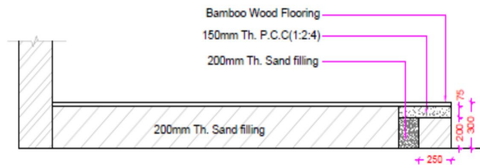
DETAILS OF STAGE FLOORING
