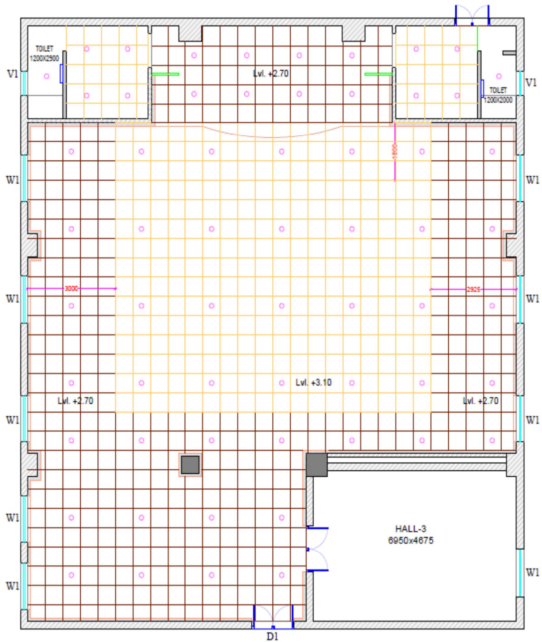
FALSE CEILING LAYOUT PLAN
