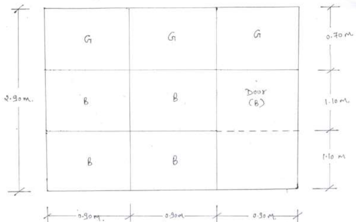
CROSS SECTION
