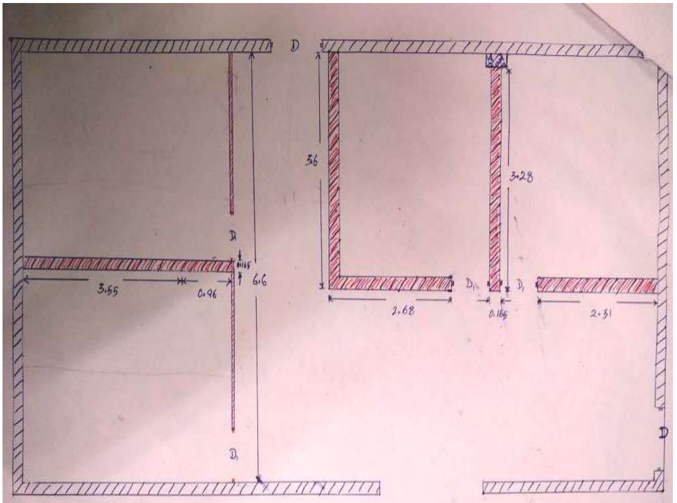
PLAN FOR REMOVAL OF EXISTING PARTITIONS
